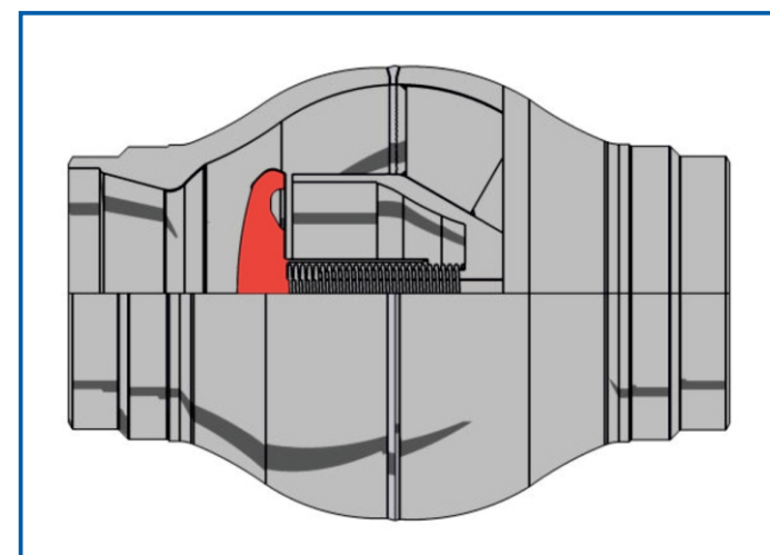
Check valve in open position
