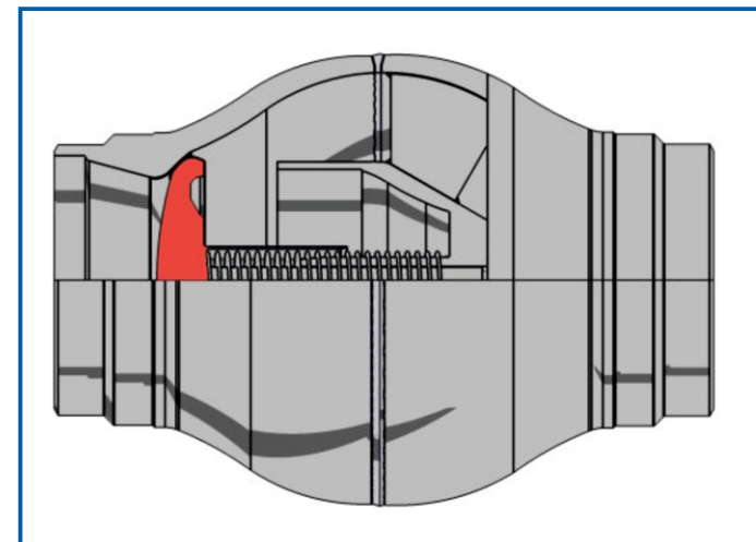
Check valve in closed position
